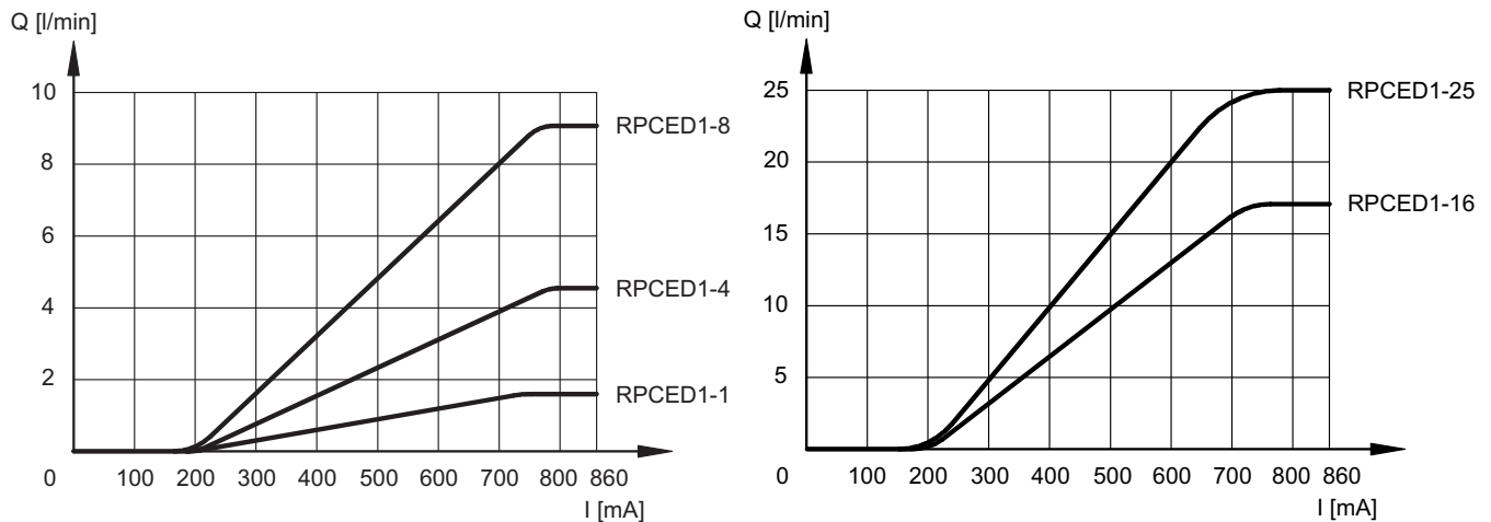
FLOW CONTROL Q=f(I)
